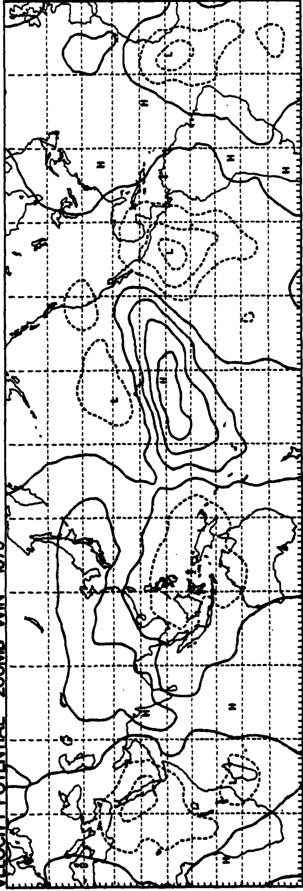
VELOCITY POTENTIAL 200MB WIN 1979
